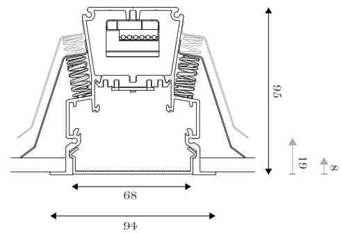
Recessed Aria LED Luminaire weight approx. 3.2 kg/m Cutout approx. 12mm shorter and narrower than overall length and width of luminaire
