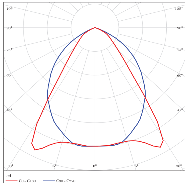
Aria LED with Louvre
