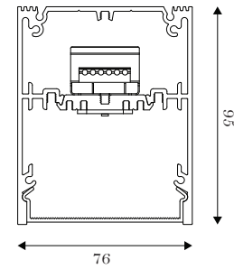
Aria LED Luminaire weight approx. 3.2 kg/m
